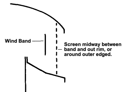
Figure 4 Proper Location of Spark Arrester Screen in Cap
